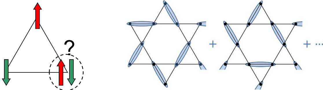
Left: frustration of the antiferromagnetic interaction on a triangular lattice. Right: one possible spin liquid state on the kagome lattice. The ellipses represent singlet states of two paired spins.
