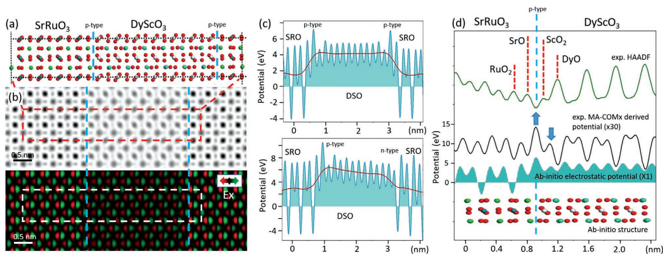
Figure 4. a) Ab-initio relaxed structural model of a -p,-p type symmetric SRO/DSO interface, with b) a corresponding electrostatic potential images and electric field component across the interface (Ex). c) ab-initio electrostatic potential profiles for two interfaces models (-p,-p type interface and -p,-n type interface) with two different spatial filtering (red and blue-cyan plain curves). The spatial filtering for the red curve has been set to vanish out the atomic-scale variations of the electrostatic potentials. d) Comparison between 4D-STEM experiments and ab-initio calculation of a n-type interface. HAADF-STEM profile and the 4D-STEM atomic-scale potential profiles are compared to the ab-initio electrostatic potential and the relaxed atomic model. The two blue arrows indicate where the potential increase and decrease in the left and right part of the interfacial unit-cell around the last Sc plane. The Sr, Ru, Sc, Dy and O atoms are, respectively, in green, blue, white, cyan and red. Please note that the ab-initio profile is the electrostatic potential while the 4D-STEM profile is the TDS potential. Both are sensitive to a FE structural distortion at the interface unit cell.
